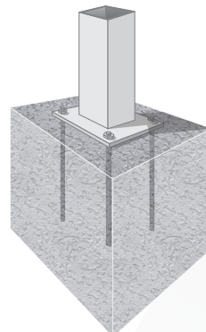
Welded plate at bottom with threaded rods into concrete
