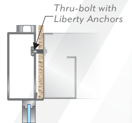
Steel Lintel Mounting
