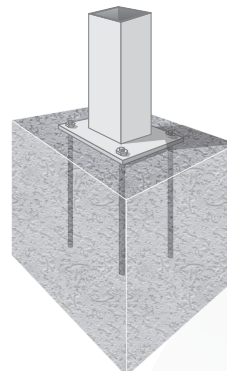
Welded plate at bottom with threaded rods into concrete
