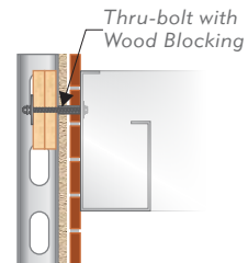
Stud Wall Mounting
