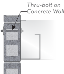
CMU Wall Mounting
