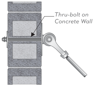
CMU Wall Mounting
