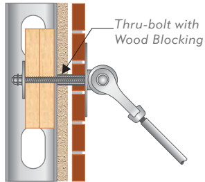
Stud Wall Mounting
