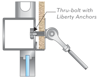
Steel Lintel Mounting
